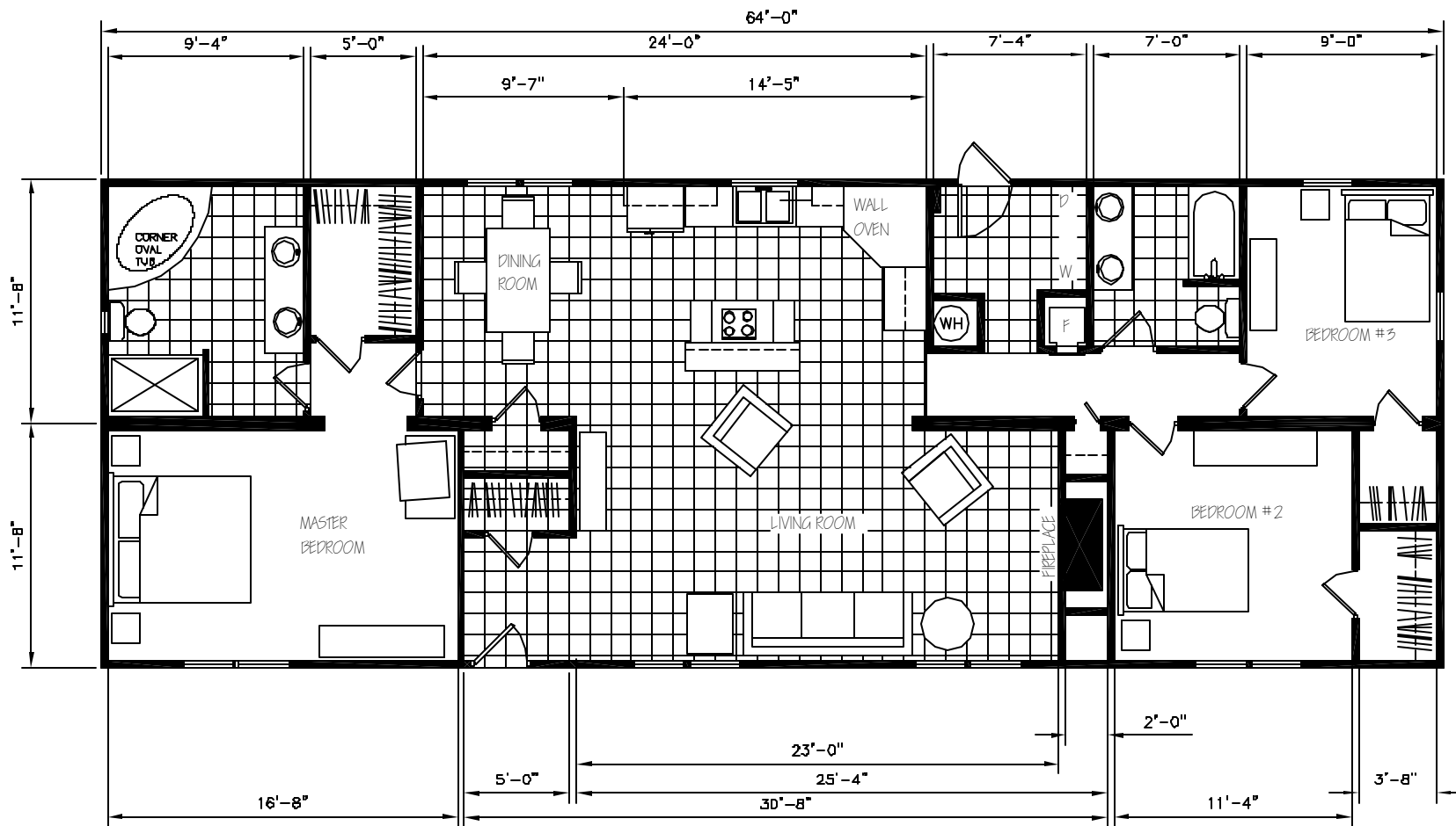
24x64 3+2 ASD HOUSE NO. 40229 APPROX. 1493 SQ. FT.
