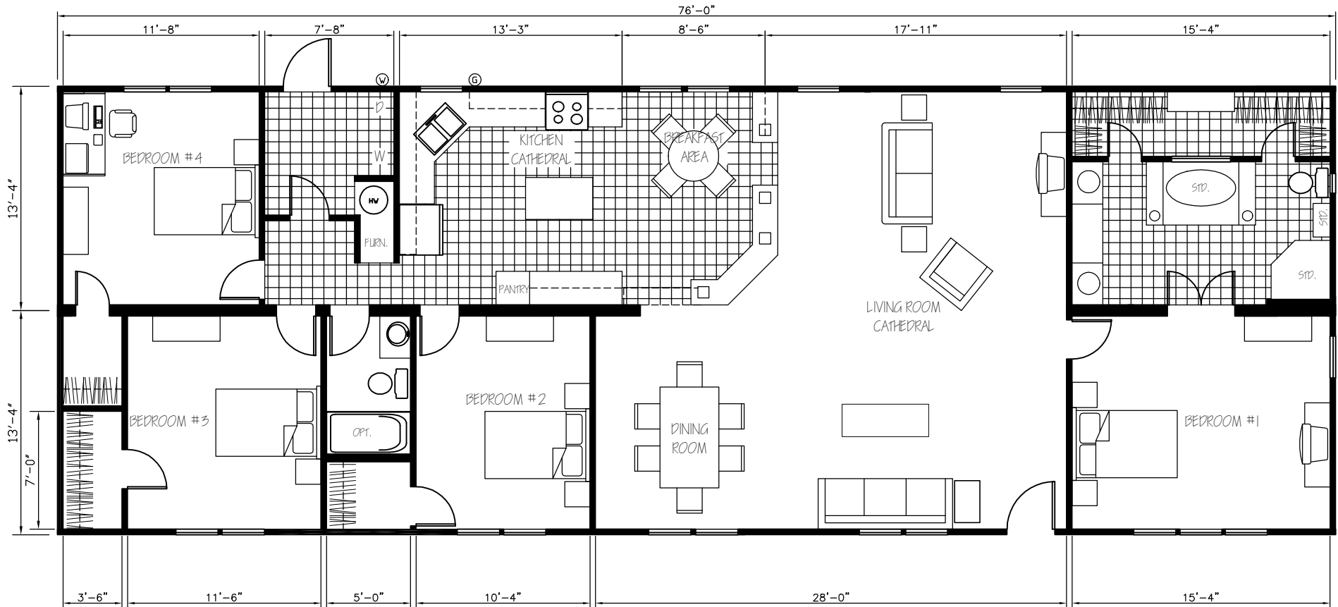
27x76 4+2 L5TP HOUSE NO. 40204 APPROX. 2026 SQ. FT.
